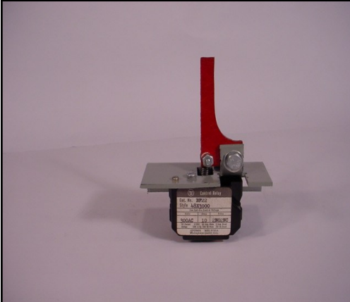
Allis Chalmers Motor Cut Off Switch for 5 & 15 KV Breakers
